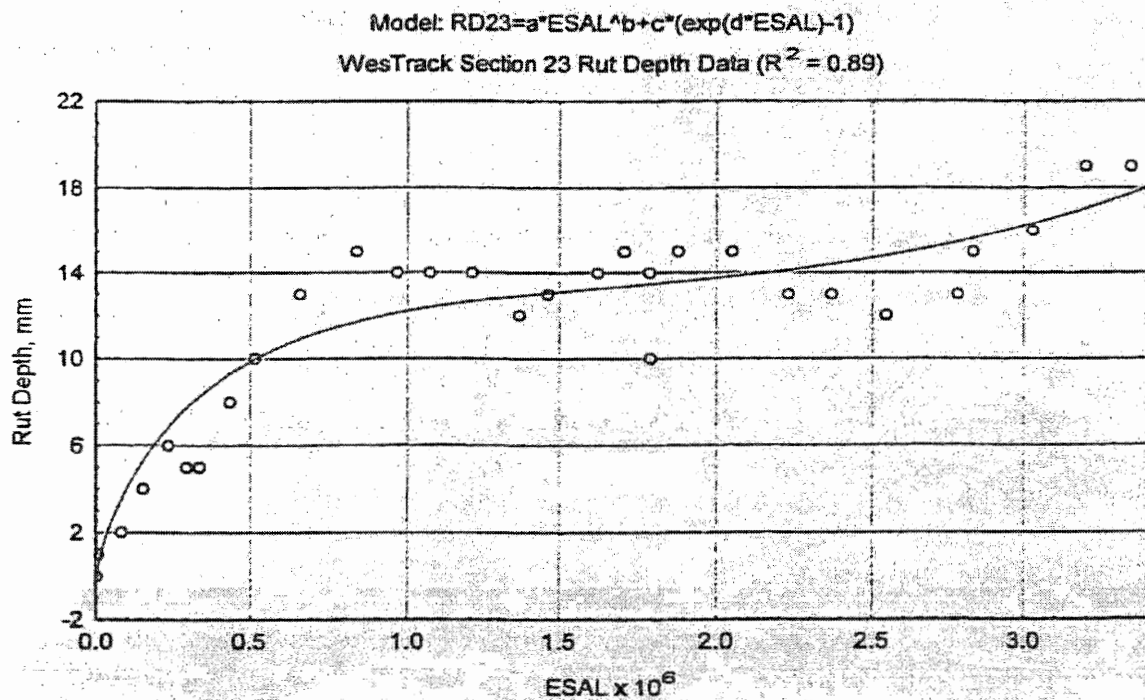
Figure 2 – Permanent Deformation at WesTrack
