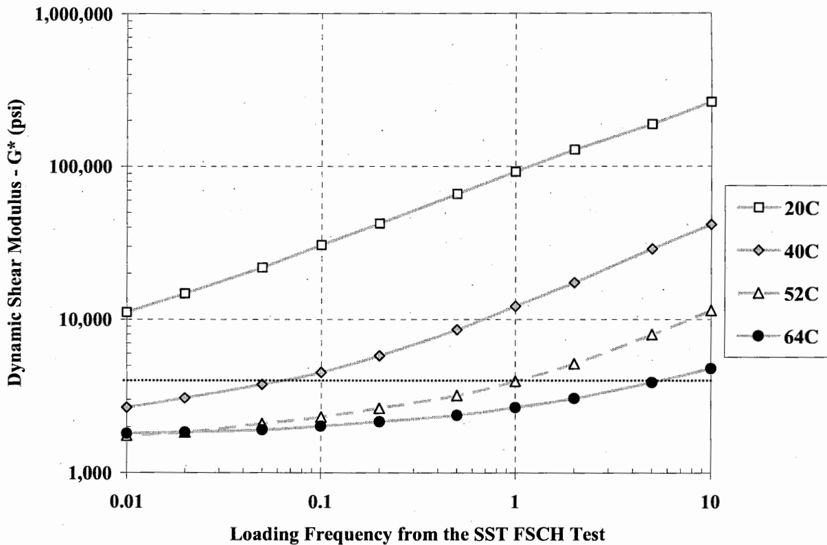
Figure 10 – FSCH Results from Testing Conducted at RAPL
