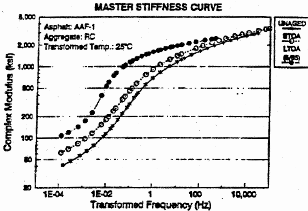
Figure 3 – Effect of Aging (Short Term and Long Term) on the Master Curve (Stiffness) of HMA
