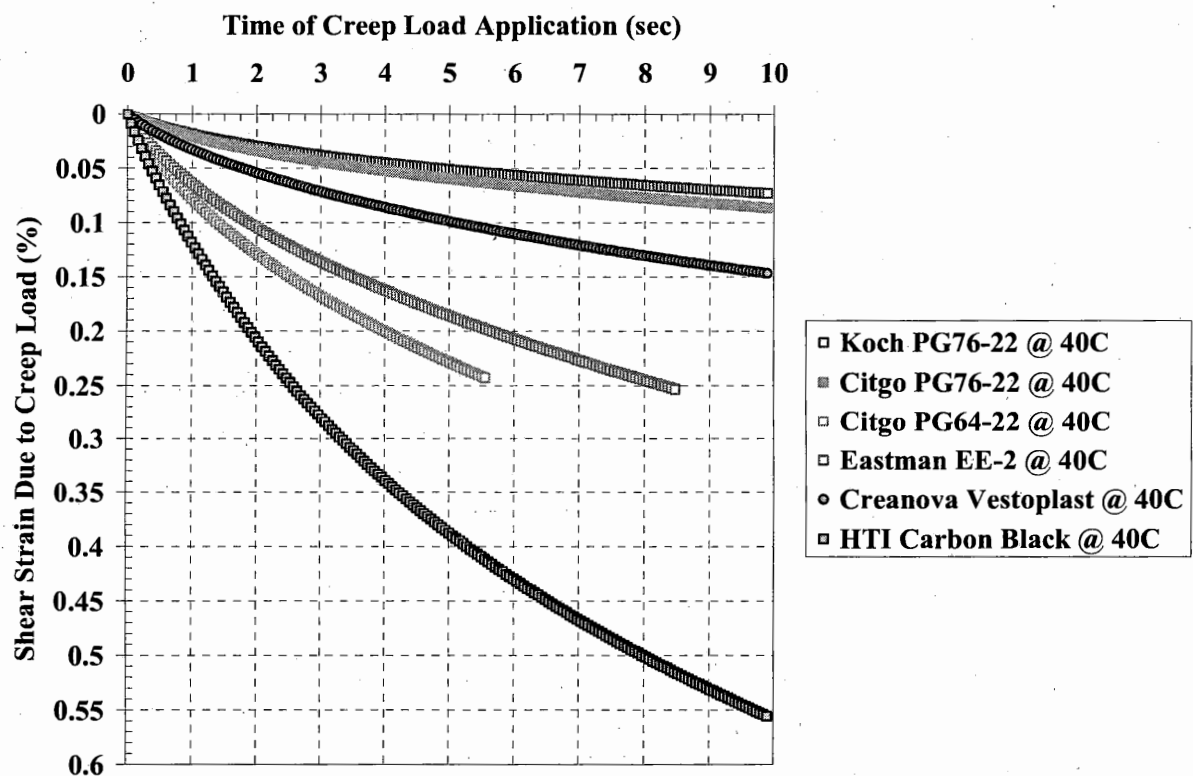
Figure 54 – SSCH Creep Curves Tested at 40°C
