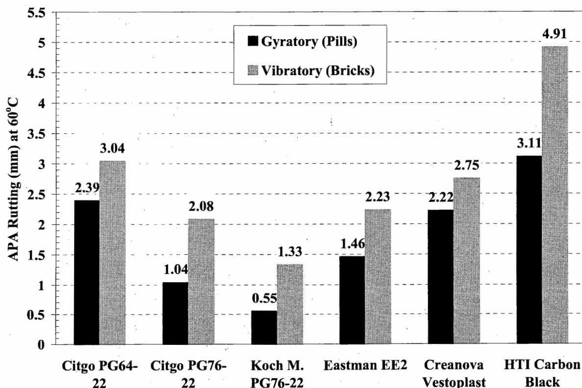
Figure 55 – Asphalt Pavement Analyzer (APA) Rutting Results
