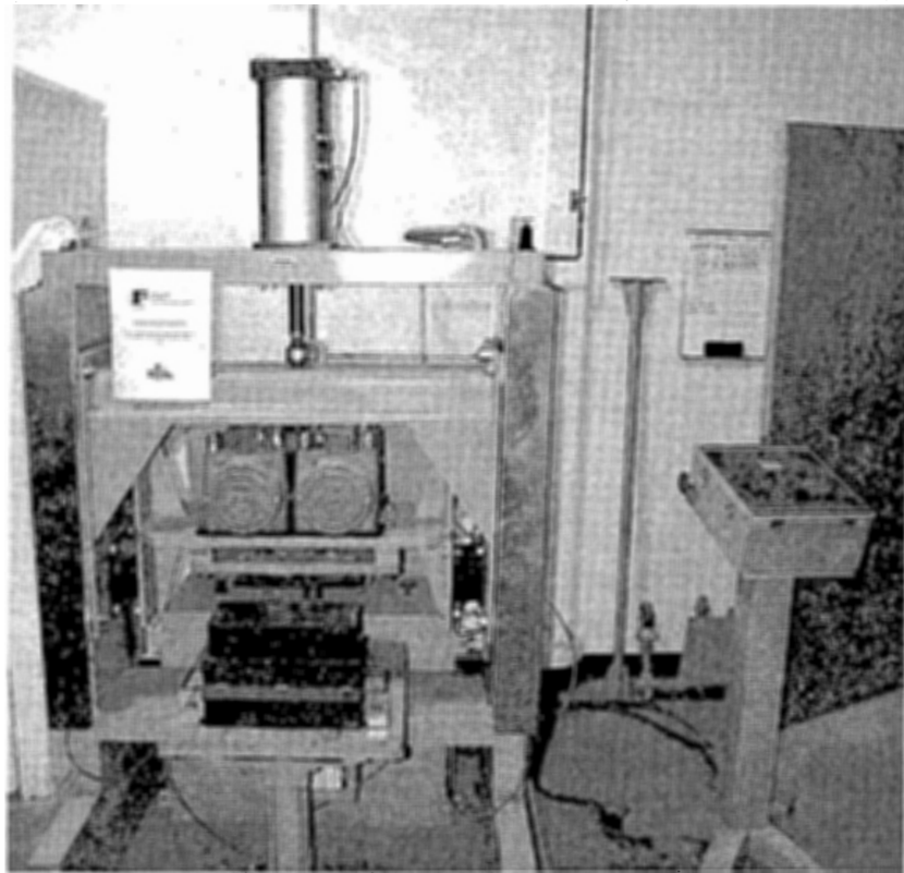
Figure 18 – Vibratory Compactor at RAPL (Manufactured by Pavement Technologies Inc.)
