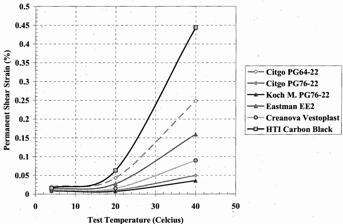
Figure 51 – Permanent Shear Strain from Simple Shear at Constant Height Test
