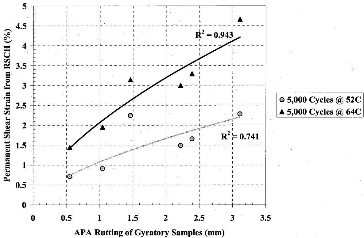
Figure 57 – APA Rutting of Gyratory Samples vs RSCH Test Results
