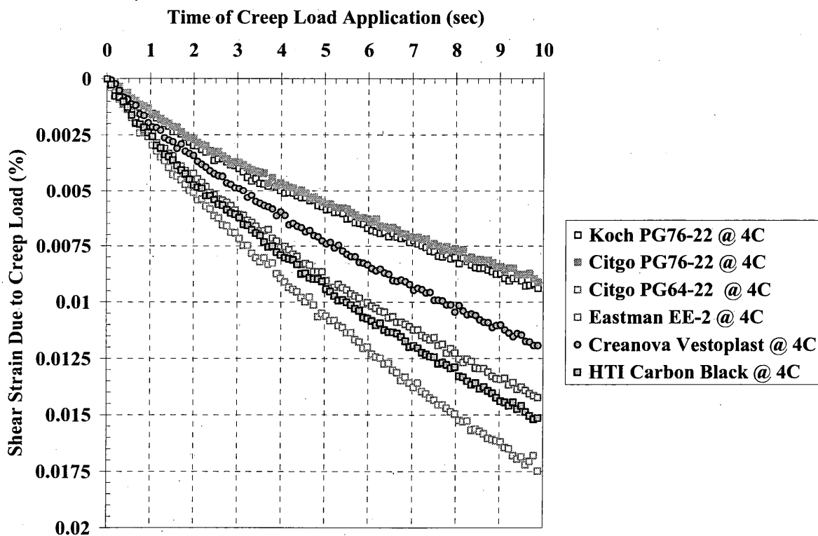
Figure 52 – SSCH Creep Curves Tested at 4°C
