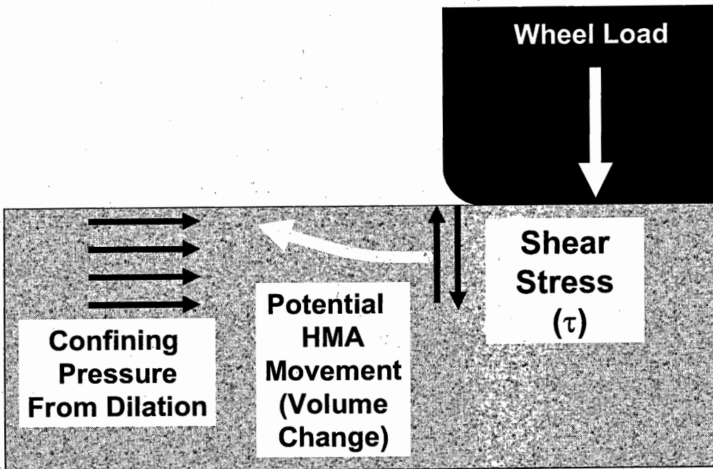
Figure 4 – Mechanism for Dilation to Occur in HMA
