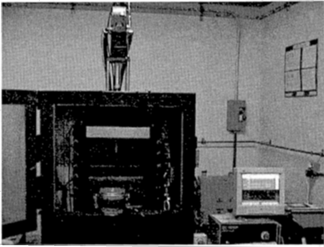
Figure 6 – Superpave Shear Tester (SST) at the Rutgers Asphalt/Pavement Laboratory
