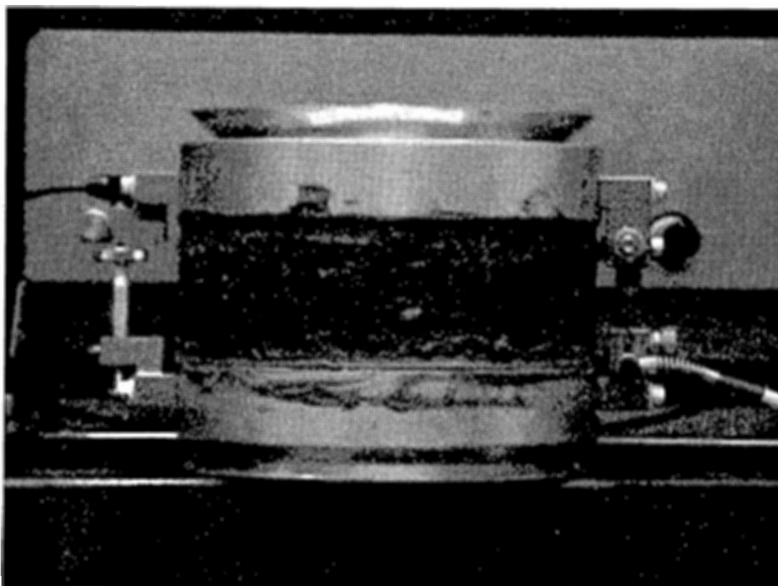
Figure 8 – SST Specimen Glued to Caps with LVDT's Attached
