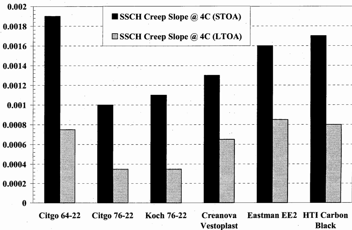
Figure 91 – Creep Slope of Aged and Unaged Samples from SSCH @ 4C
