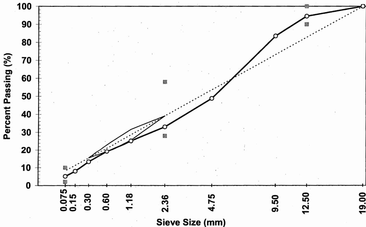
Figure 15 – Mix Design Gradation Used for 12.5mm Superpave Design
