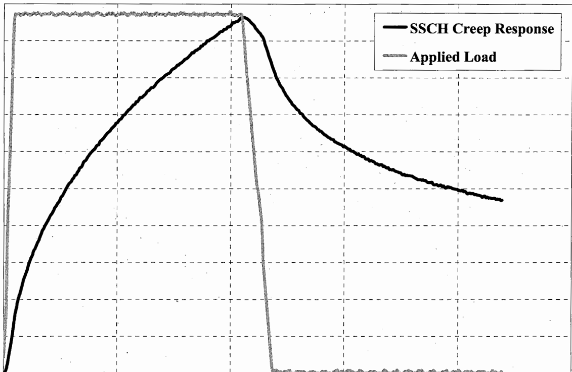
Figure 46 – Typical SSCH Sample Response and Applied Load at 40°C
