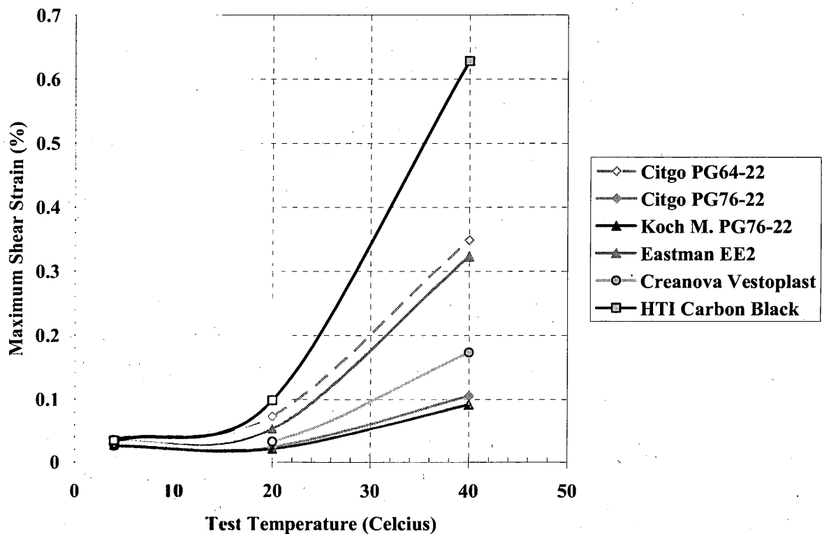
Figure 50 – Maximum Shear Strain from Simple Shear at Constant Height Test
