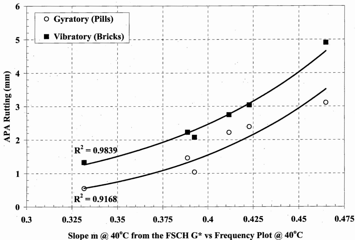
Figure 63 – FSCH m -Slope Parameters @ 40°C vs APA Rutting
