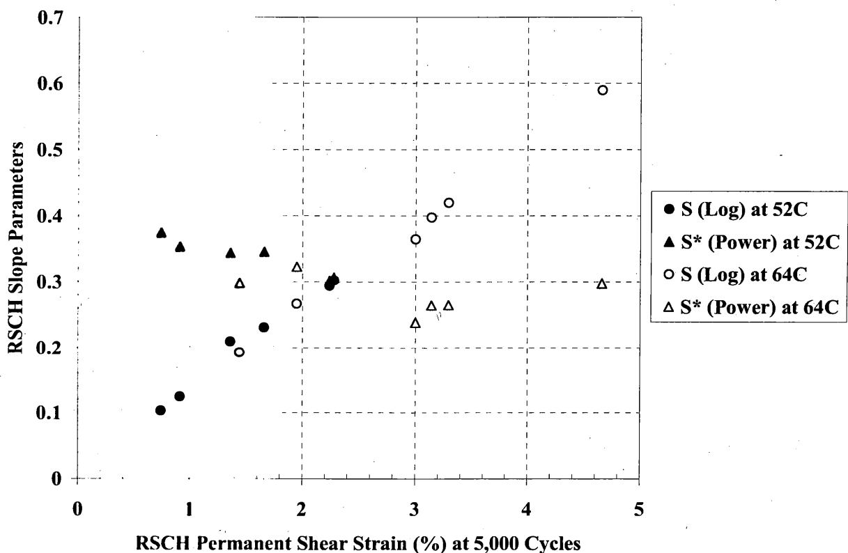
Figure 28 – Relationship Between Sloping Parameters and RSCH Permanent Shear Strain at 5,000 Loading Cycles
