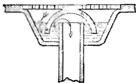
BELL TRAP.
