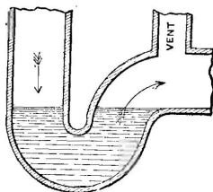
P TRAP.
