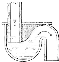
D TRAP.
