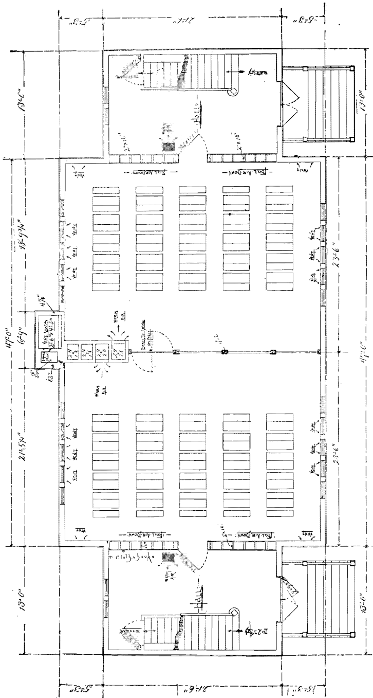
FIRST FLOOR PLAN. School House at Hopewell, Mercer County, N. J.
