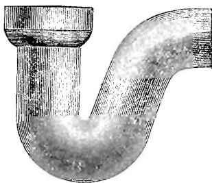
HALF-S TRAP.
