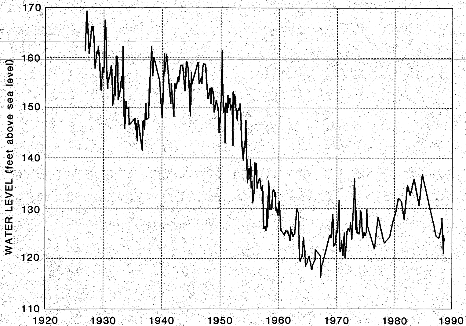
Figure 6. Hydrograph of the Neutral Zone observation well, 1926-1988. Source: Files of the New Jersey Geological Survey and U.S. Geological Survey. (U.S.G.S. Well ID 13-0014) Land surface elevation = 179'.
