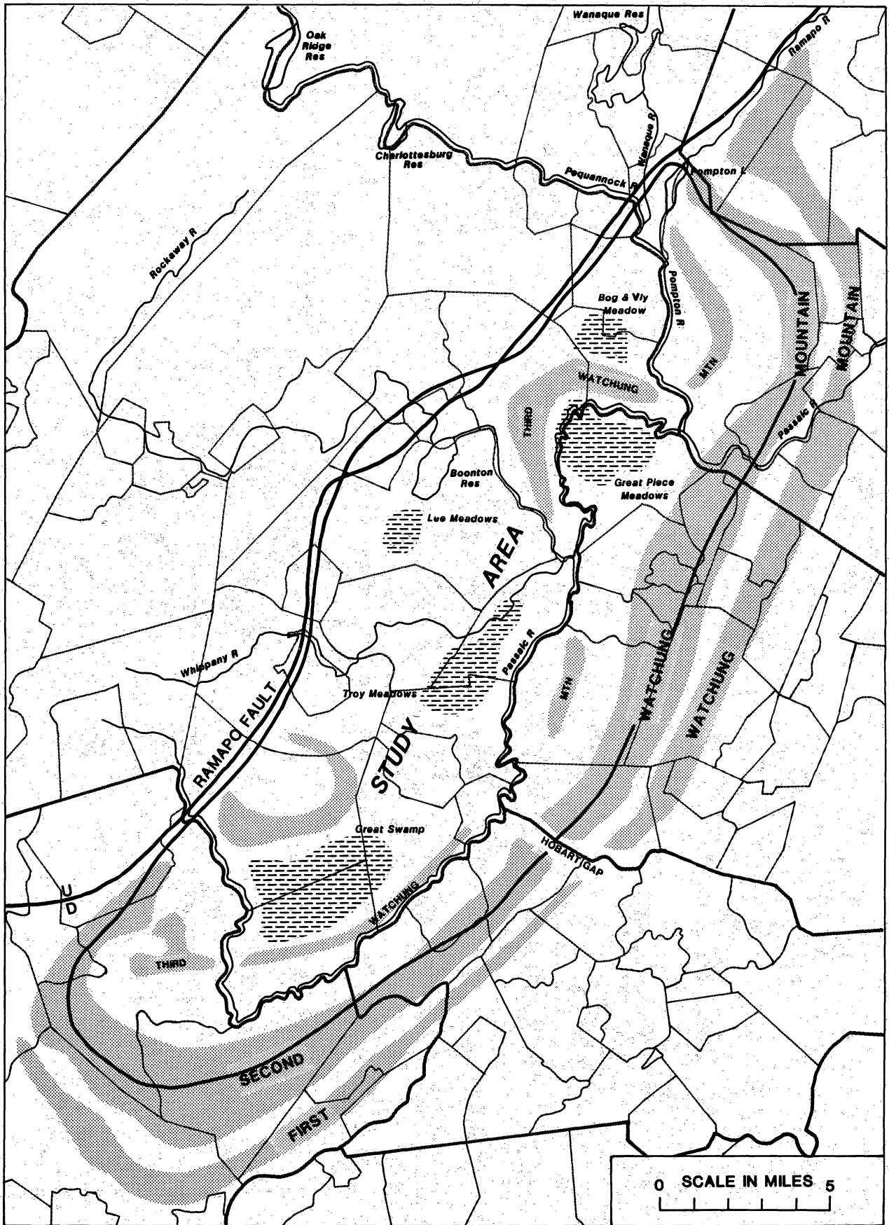
Figure 2. Major geographical features of the Central Passaic River Basin. Geology from Olsen (1980).
