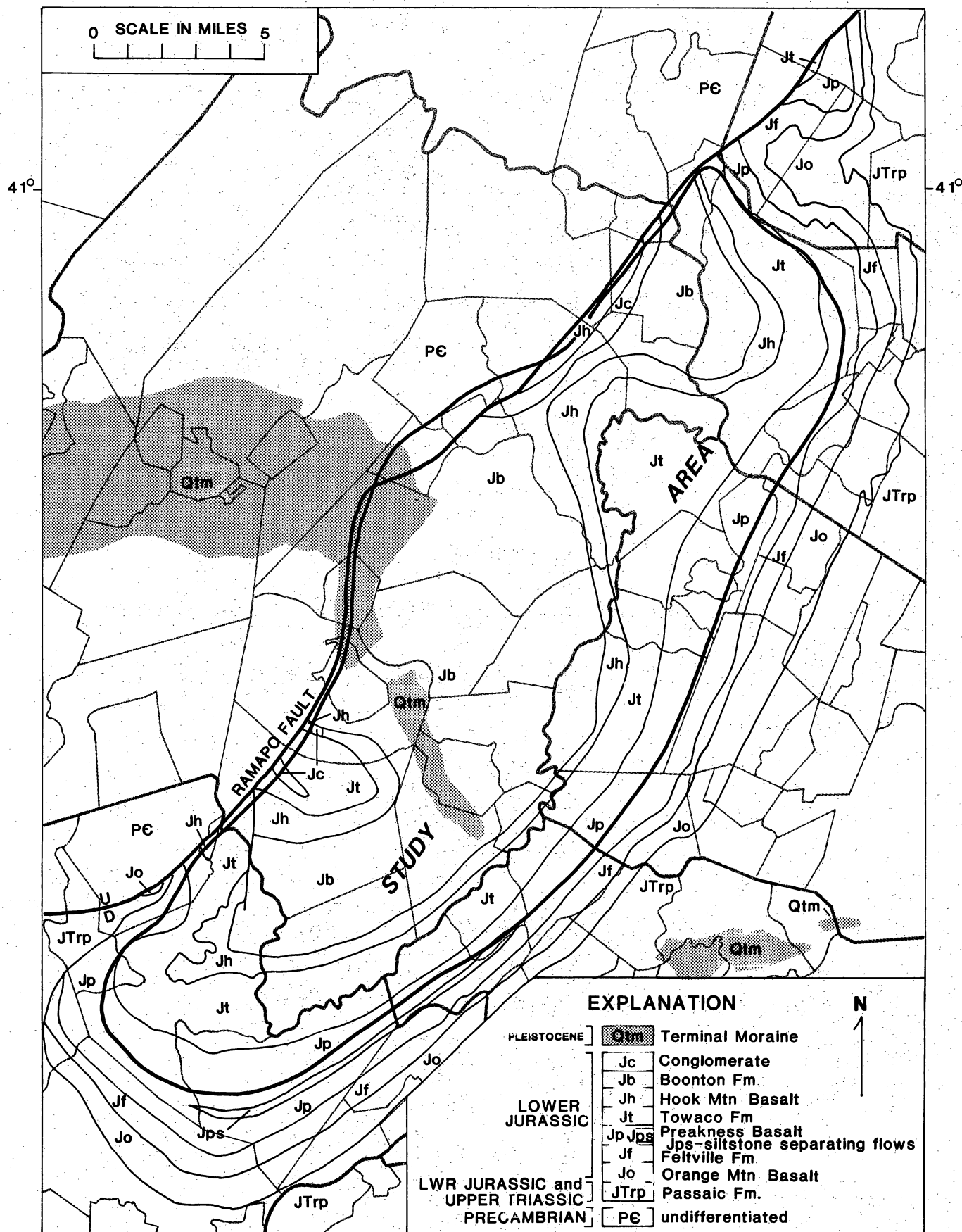
Figure 7. Generalized bedrock geology and terminal moraine. Bedrock geology south of 41° latitude modified from Lyttle and Epstein (1987), remainder from Houghton (personal communication, 1988). Terminal moraine from Lewis and Kummel (1912).
